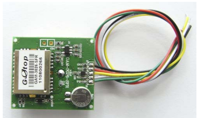
GAM-3026-SFR Top View&Bottom View
